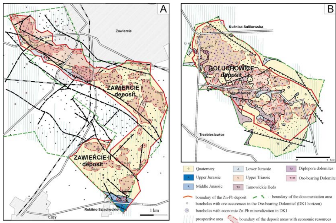
Fig. 2A–B. Map of Zn-Pb sulfide mineralization in the Ore-bearing Dolomite in the DK1 horizon in the Zawiercie I, Zawiercie II (A) and Gołuchowice deposits (B), after Mikulski et al. (2010) with Zn-Pb ore prospective areas
